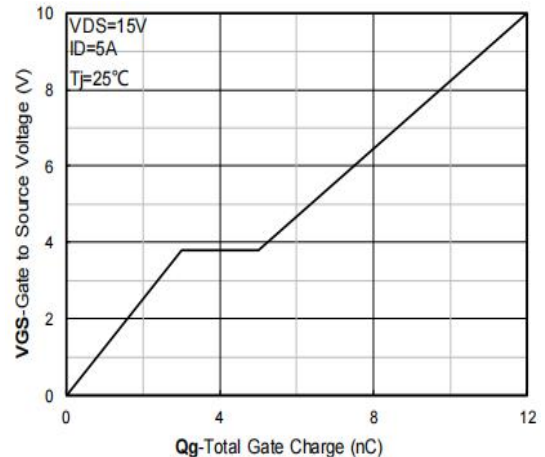
Figure 6: Gate-Charge Characteristics
