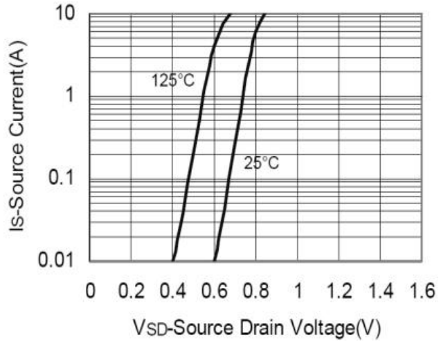
Figure 8: Diode Characteristics
