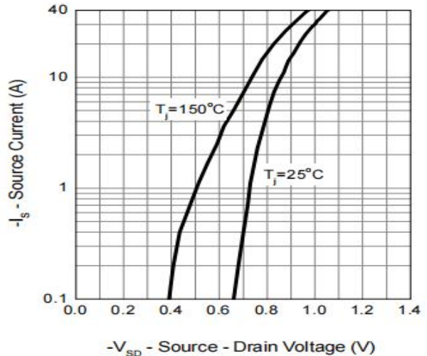
Figure 8: Diode Characteristics
