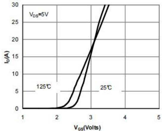
Figure 4: Transfer Characteristics
