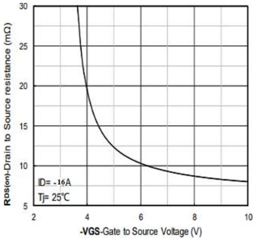
Figure 7: On-Resistance vs. V_{GS}
